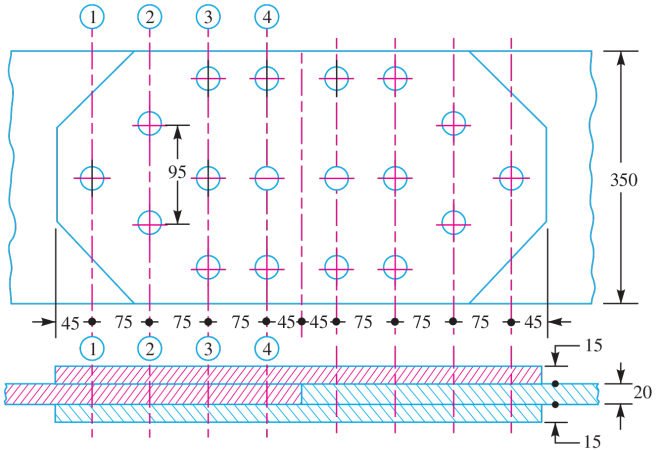
Fig. 9.21. All dimensions in mm.
